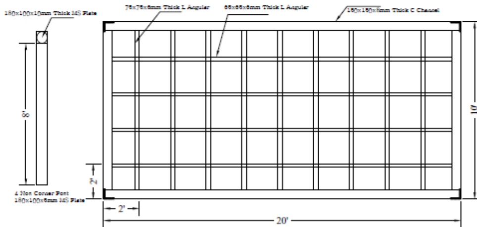
20'x10'x8' Shipment Toilet Portacabin Bottom Framing
