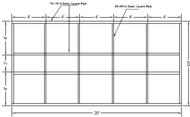
20'x10'x8' Shipment Toilet Portacabin Top Framing
